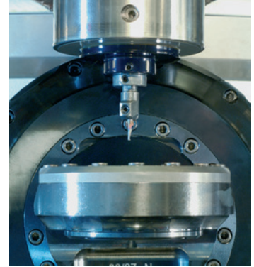
RH Spindle, ideal for precise recessing.
